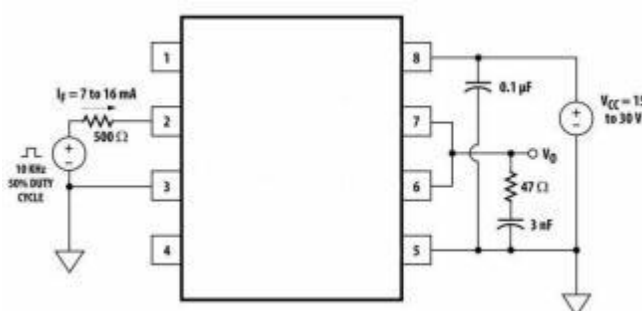
Fig.16 I_{FIH} test circuit
