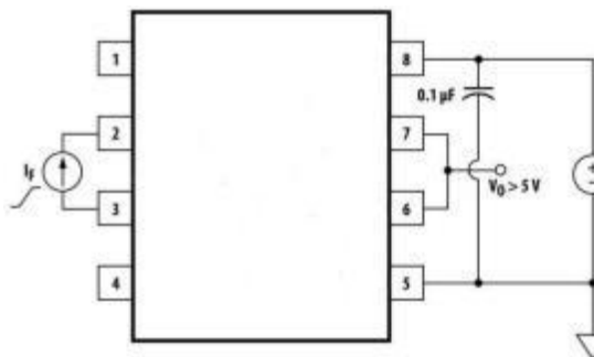
Fig.16 I_{FIH} test circuit
