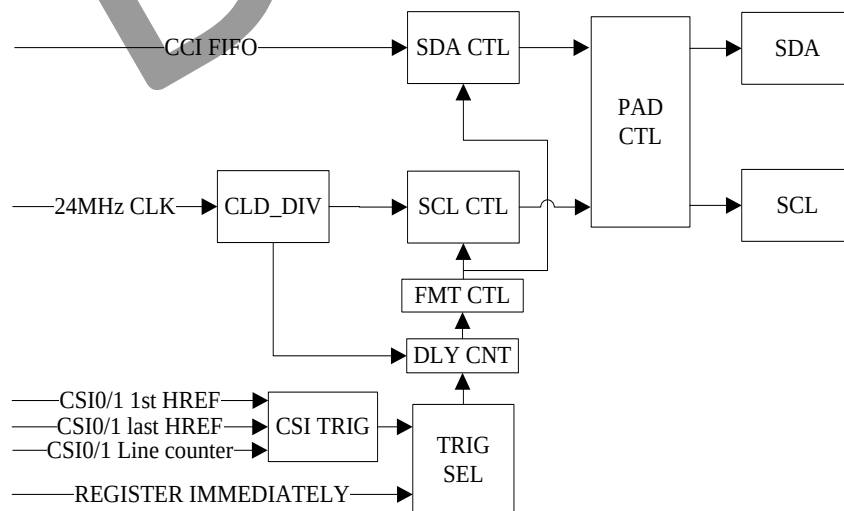
Figure 6-2. CCI Block Diagram
