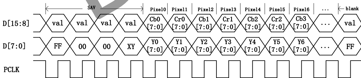
Figure 6-4. 16bit YCbCr4:2:2 with separate syncs Timing (clock rising edge sample.vsync valid = positive,hsync valid = positive)
