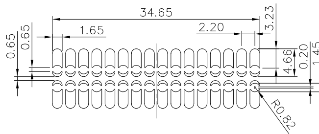
STEEL MESH (BOTTOM SIDE) T \geq 0.12\text{mm}
