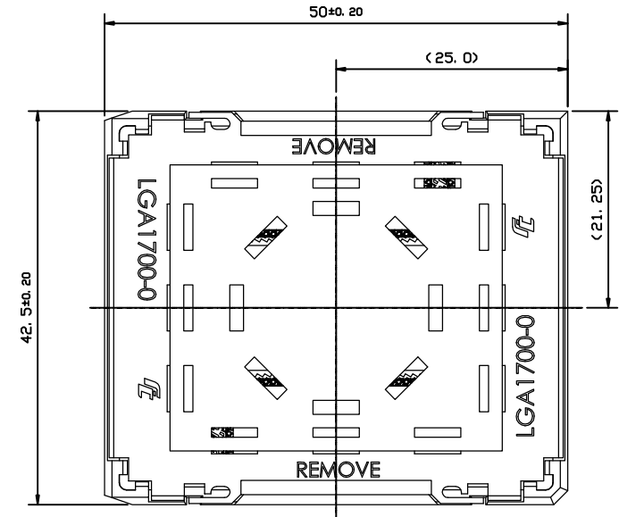
SOCKET W/ CAP (TOP VIEW)
