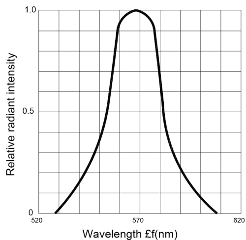
Fig.1 Relative intensity vs. Wavelength
