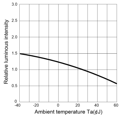
Fig.4 Relative luminous intensity vs. Ambient temperature
