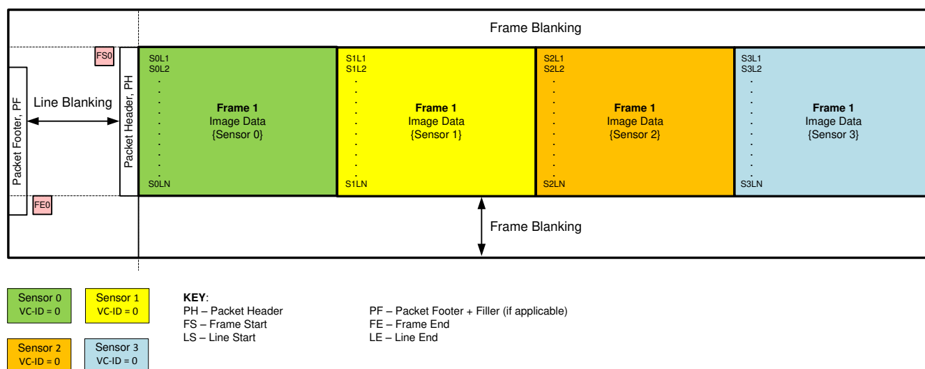
图 5-20. Line-Concatenated Format
