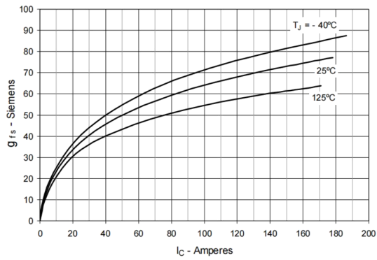
Fig. 7. Transconductance
