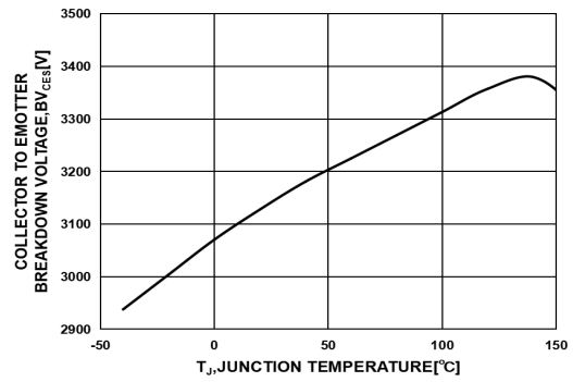
Fig. 8 Collector to Emitter Breakdown Voltage vs. Junction Temperature
