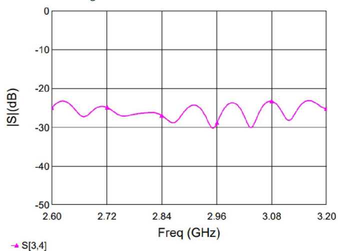
Figure 9. MHC29X03 Isolation
