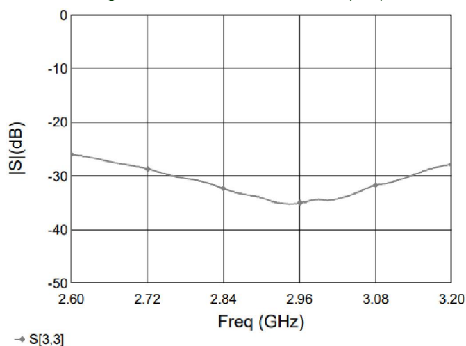
Figure 7. MHC29X03 Return Loss (S33)
