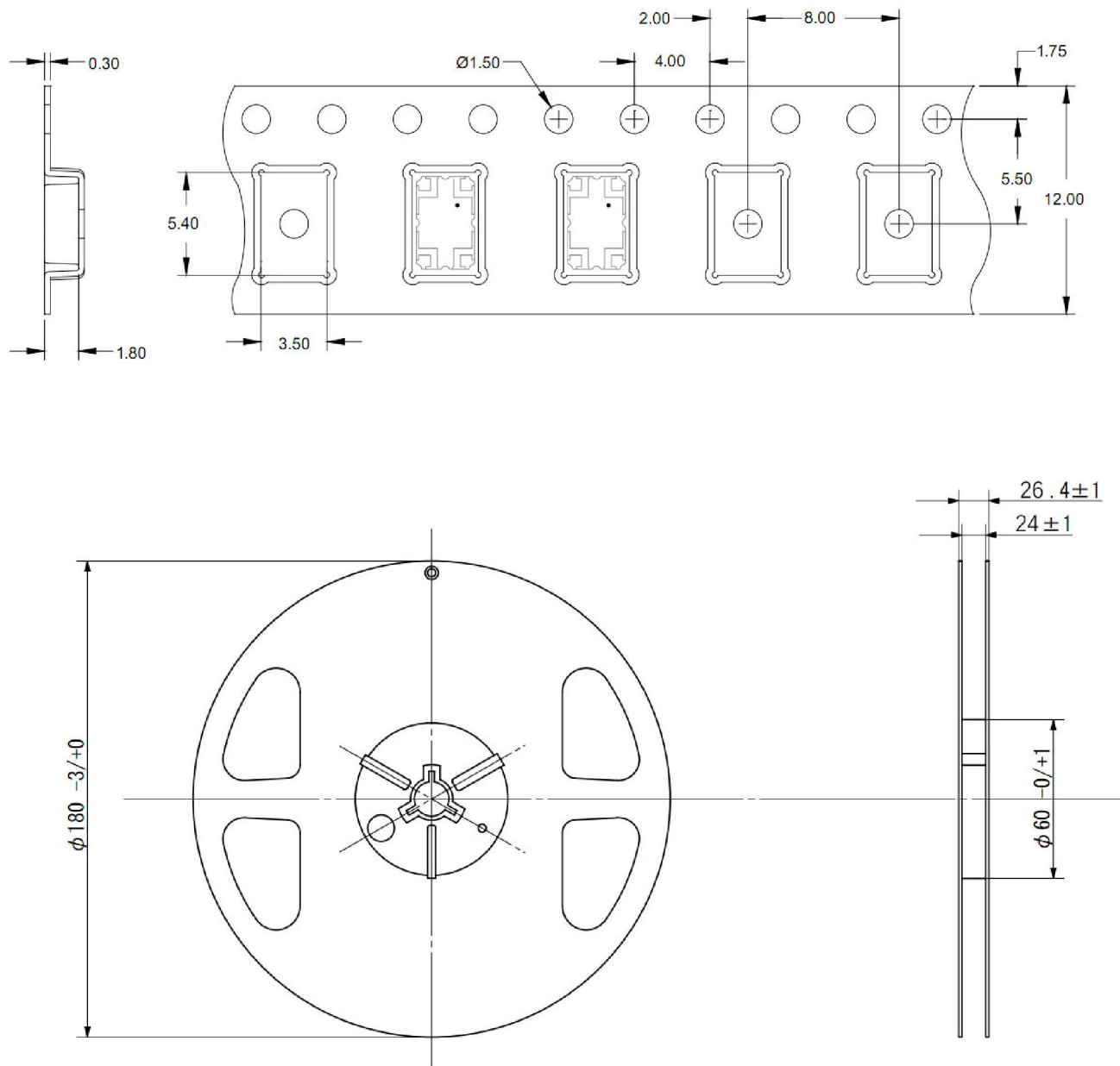
Figure 12. MHC29X03 Packaging Information
