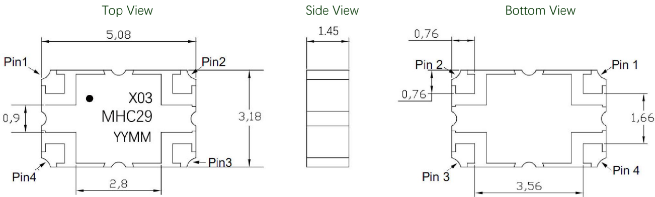
Figure 2. MHC29X03 Outline Drawing
