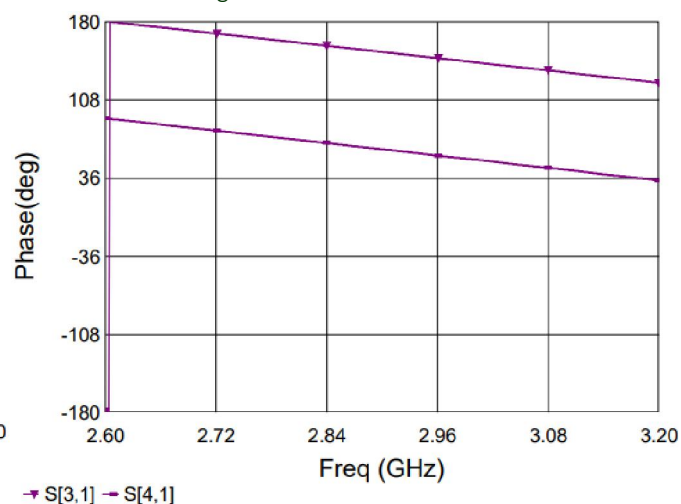
Figure 10. MHC29X03 Phase
