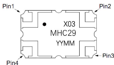
Figure 1. MHC29X03 (Top View)
