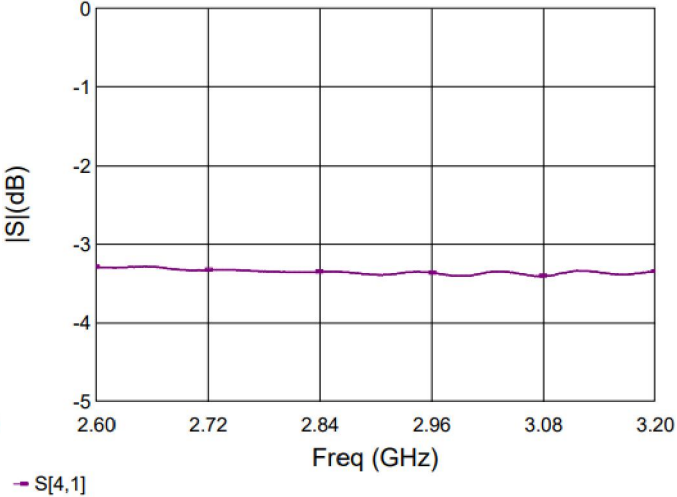
Figure 4. MHC29X03 Transmission
