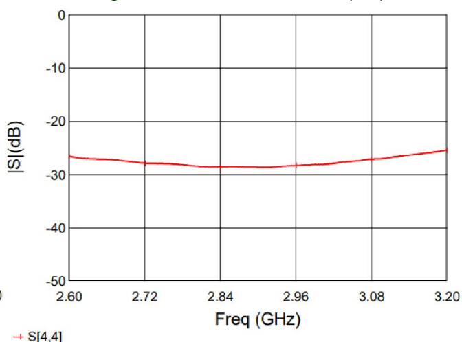
Figure 8. MHC29X03 Return Loss (S44)
