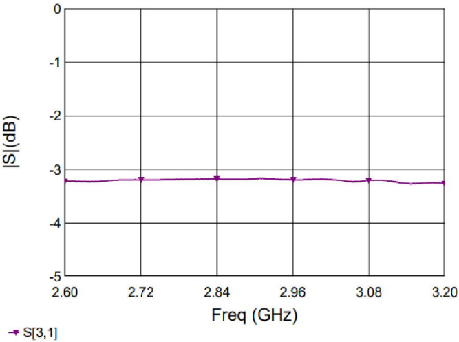
Figure 3. MHC29X03 Coupling
