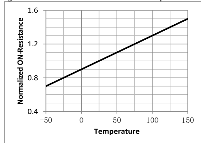
Fig.12 On-Resistance V.S Junction Temperature
