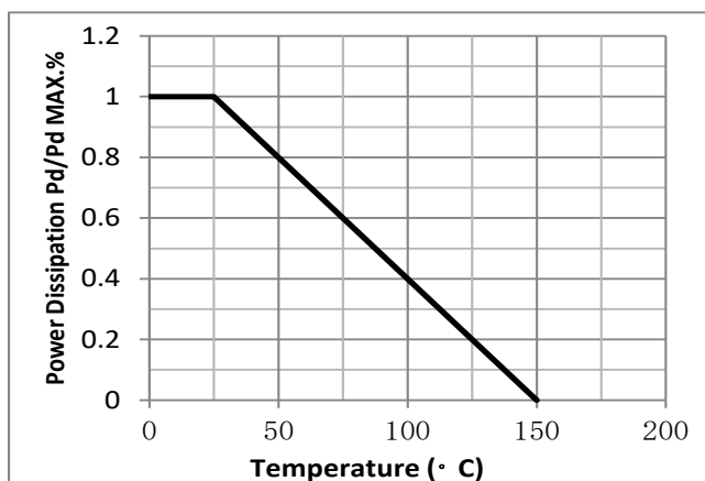
Fig.1 Power Dissipation Derating Curve
