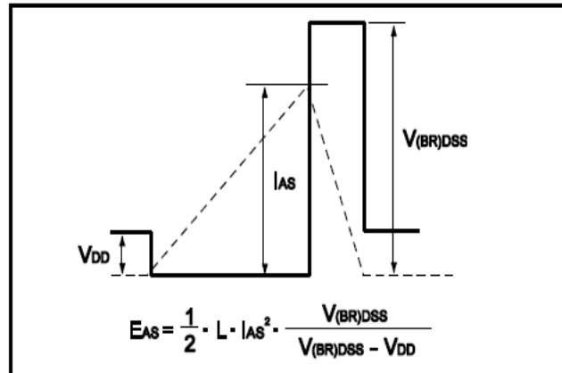
Fig.18 Avalanche Waveform
