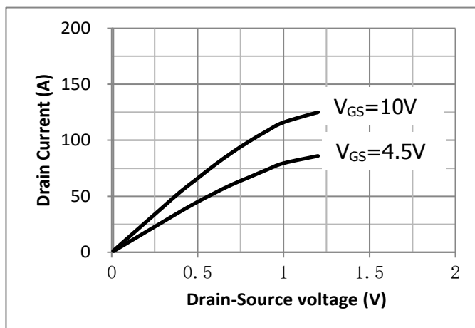
Fig.8 Typical output Characteristics
