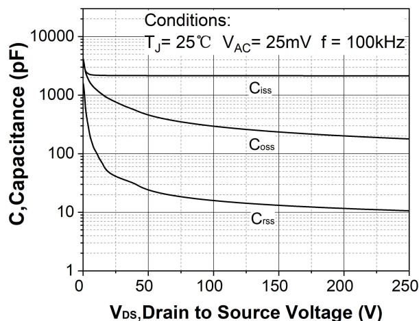
Figure 17. Capacitances vs. drain-source voltage (0 - 250V)
