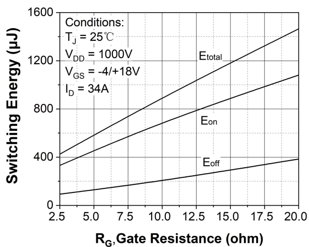
Figure 25. Clamped inductive switching energy vs. R_G(\text{ext})
