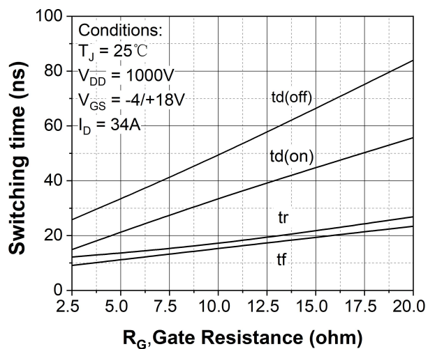
Figure 27. Switching times vs. R_G(\text{ext})
