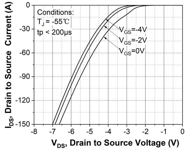
Figure 8. Body diode characteristic at T_J = -55^\circ C
