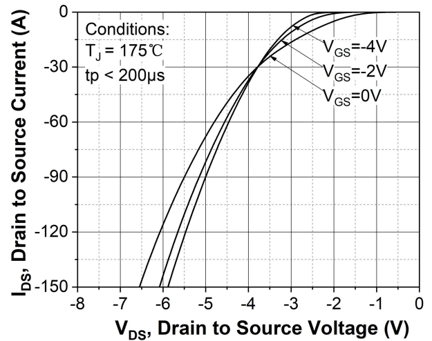
Figure 10. Body diode characteristic at T_J = 175^\circ C
