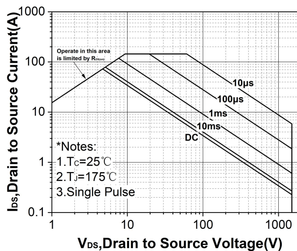
Figure 22. Safe operating area
