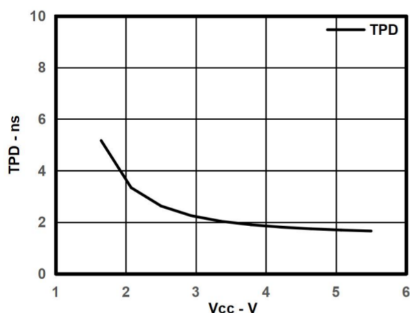
Figure 1. Typical Tpd vs Vcc
