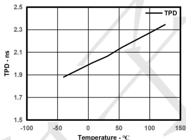
Figure 2. Typical Tpd vs Temp
