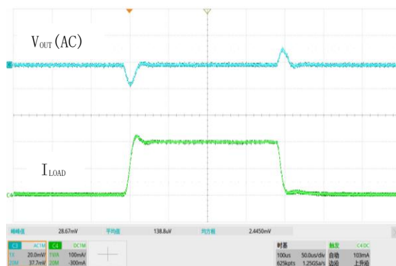
图 22. 负载瞬态响应, V_{IN}=4.3V , V_{OUT}=3.3V , I_{OUT}=1mA to 200mA
