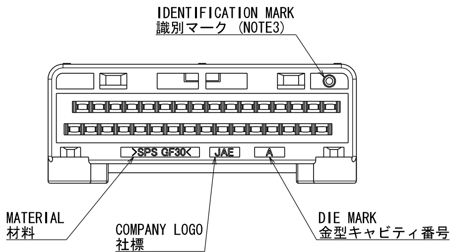
DETAIL C (HOUSING ONLY)
