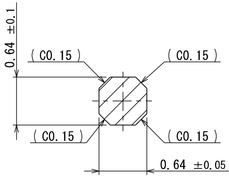
SECT. B-B (20 : 1)
