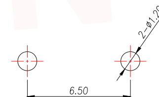
PCB.WELDING DRAWING
