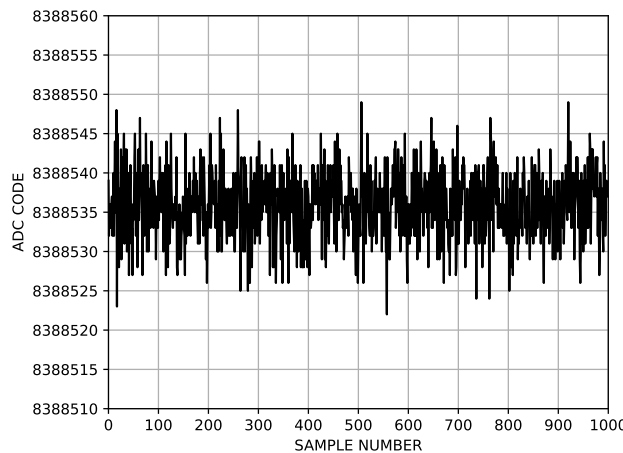
Figure 7. Noise (Analog Input Buffers Disabled, V REF = 5 V, Output Data Rate = 10 kSPS)
