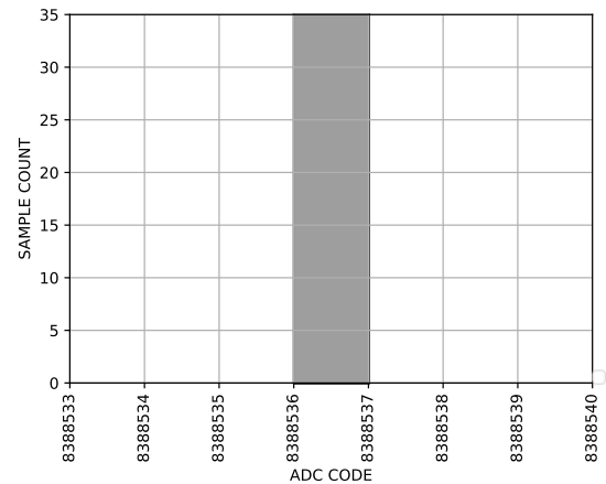
Figure 6. Histogram (Analog Input Buffers Disabled, V REF = 5 V, Output Data Rate = 5 SPS)
