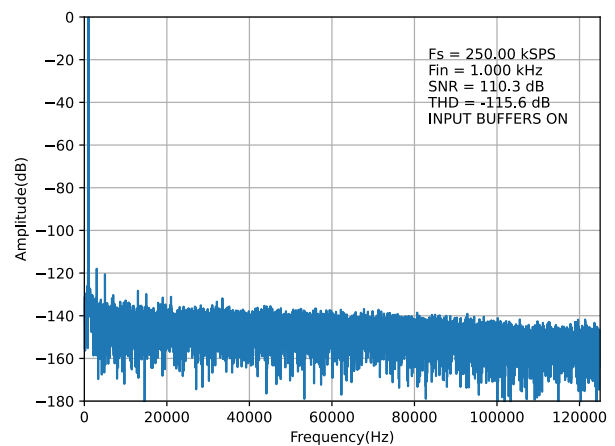
Figure 24. Full-scale FFT (INPUT BUFFERS ON, External 5V Reference)
