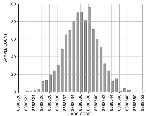
Figure 8. Histogram (Analog Input Buffers Disabled, V REF = 5 V, Output Data Rate = 10 kSPS)
