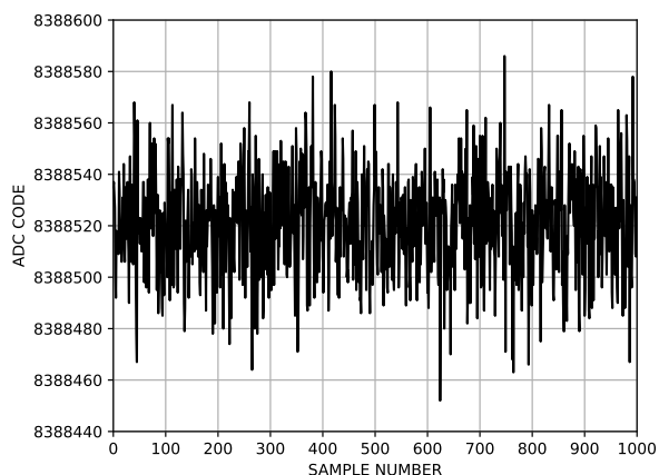
Figure 15. Noise (Analog Input Buffers Enabled, V_{REF} = 5\text{ V} , Output Data Rate = 250 kSPS)
