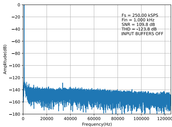
Figure 23. Full-scale FFT (INPUT BUFFERS OFF, External 5V Reference)
