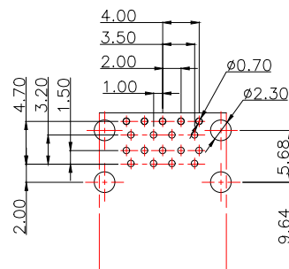
RECOMMENDED P.C.B HOLE LAYOUT TOP VIEW (TOLERANCE: ±0.05)
