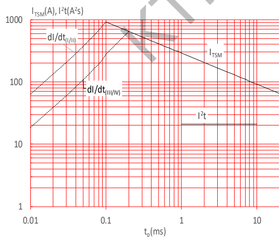
FIG.5: Non-repetitive surge peak on-state current for a sinusoidal pulse with width t_p < 20\text{ms} , and corresponding value of I^2t ( I-II: di/dt < 80\text{A}/\mu\text{s} ; III-IV: di/dt < 40\text{A}/\mu\text{s} )
