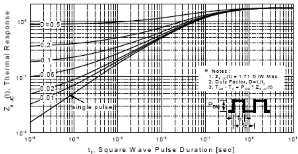
Figure 11-1. Transient Thermal Response Curve for TSP830M
