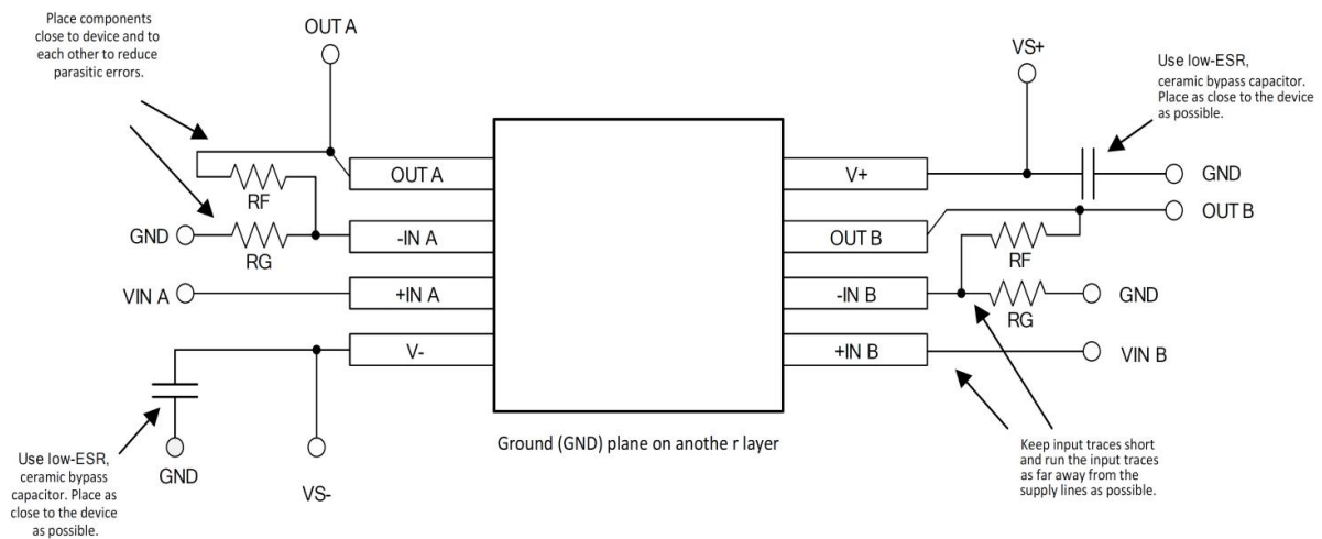
Figure 8. Layout Example
