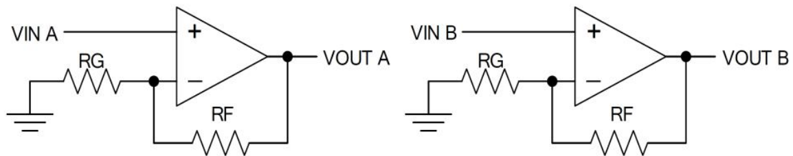
Figure 7. Schematic Representation
