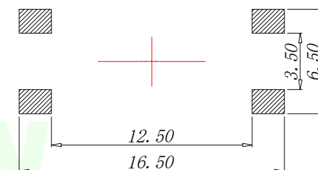
PCB.WELDING DRAWING
