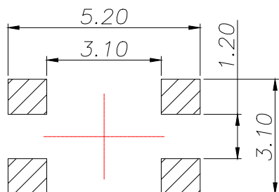
PCB.WELDING DRAWING
