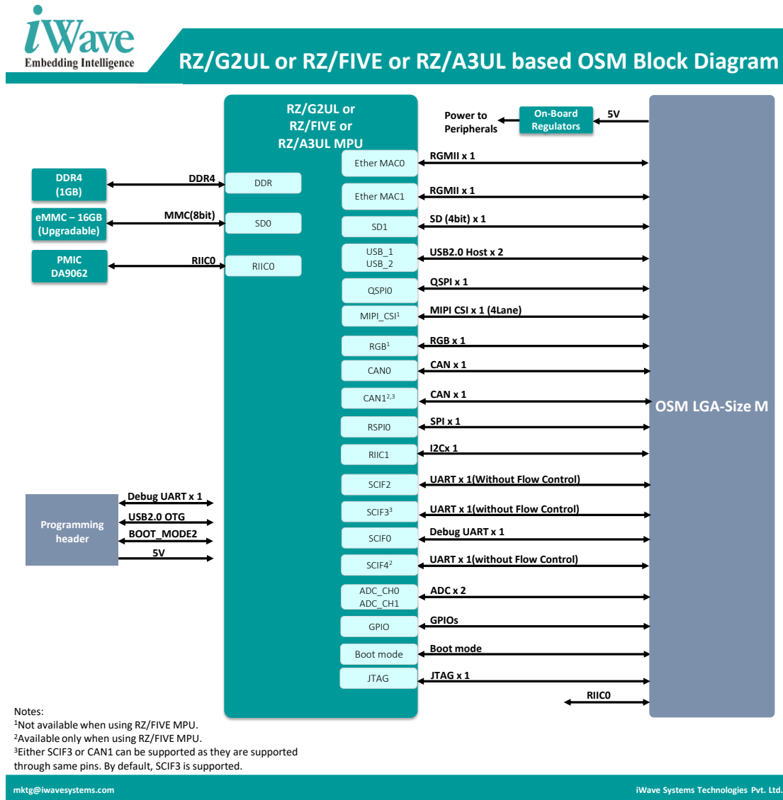
Figure 1: Renesas RZ/G2UL, RZ/FIVE or RZ/A3UL OSM LGA Block Diagram
