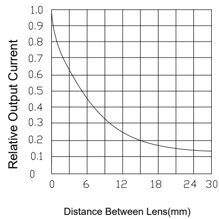
FIG.2 Coupling Characteristics
