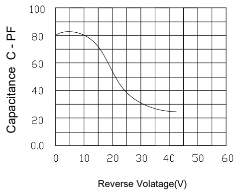
FIG.4 VR vs CT
