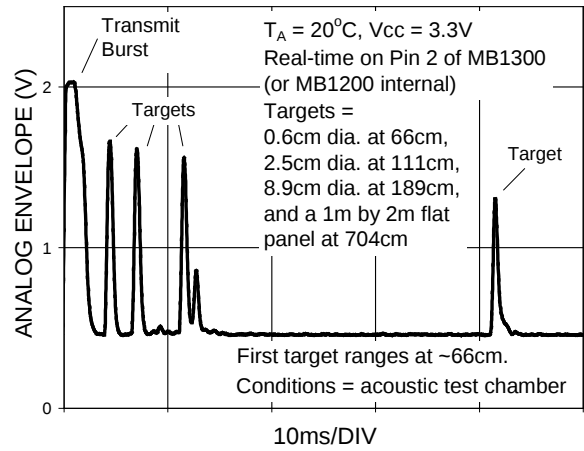
Analog Envelope Output (Dowels, 3.3V)
