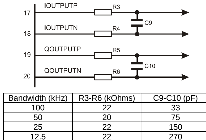
Figure 10 Recommended External Components – I/Q Output Reconstruction Filter
