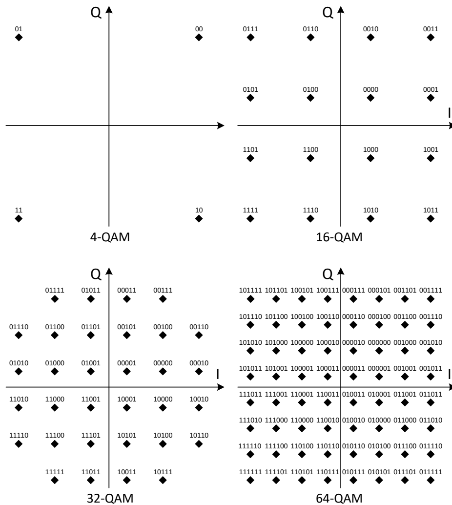
Figure 82 QAM Mappings
