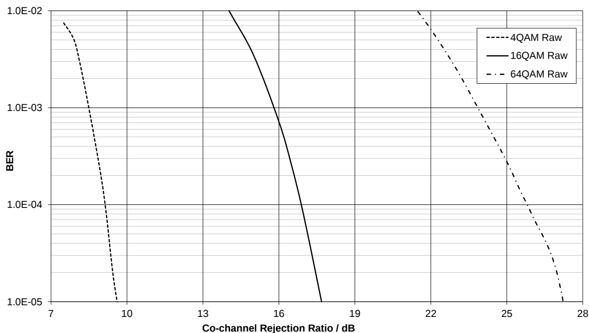
Figure 93 Modem Co-channel Rejection with FM Interferer (as EN 300 113)
