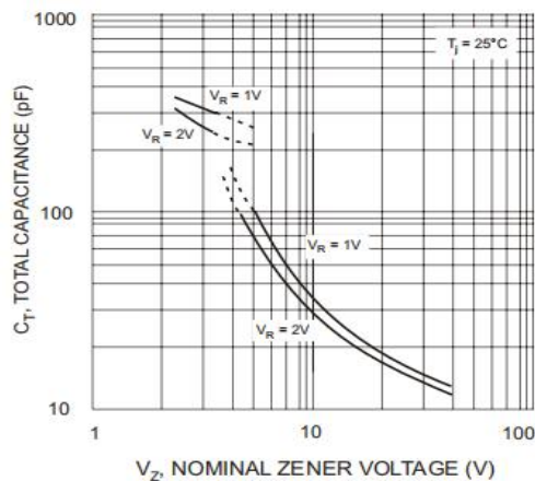
Figure 4: Capacitance Characteristics
