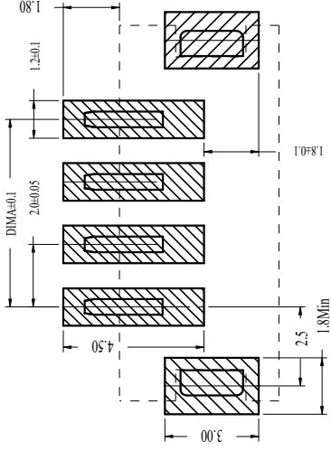
PCB LAYOUT
