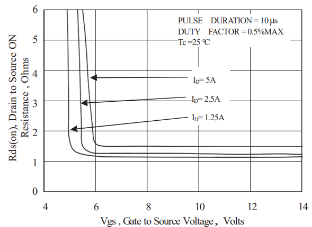
Figure 8 Typical Drain to Source ON Resistance vs Gate
