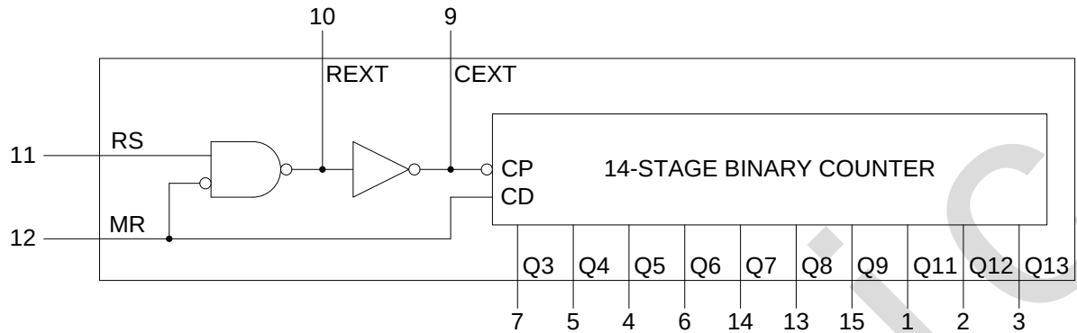
Figure 1. Functional diagram
