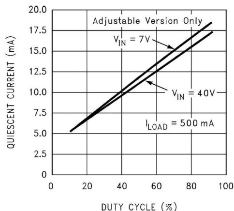
Quiescent Current vs Duty Cycle
