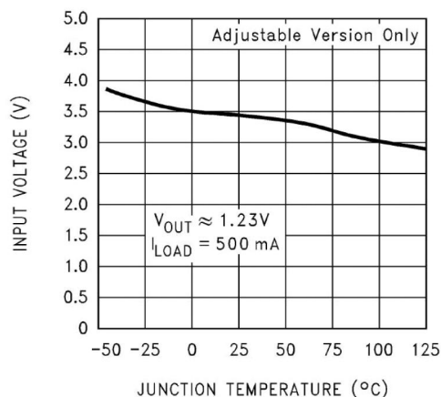
Minimum Operating Voltage
