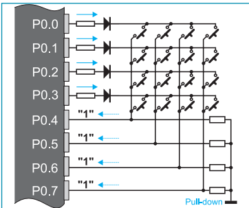
Figure 12-2: 4x4 keypad performance
