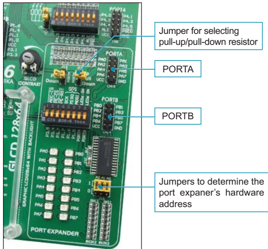
Figure 18-1: Port expander
