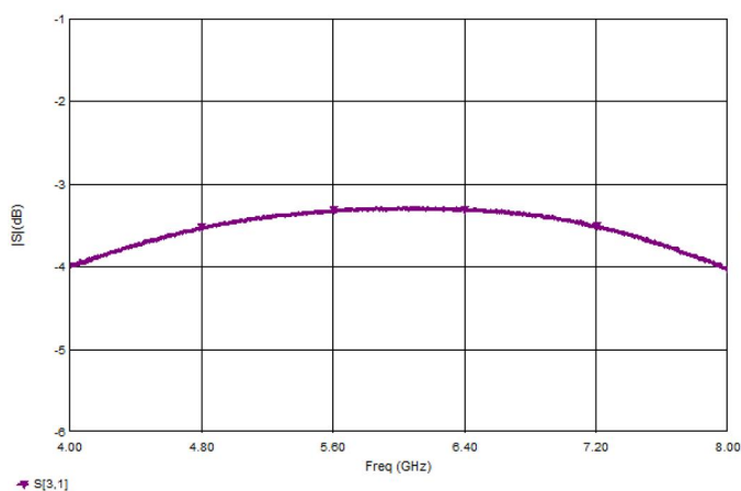
Figure 3. MHC60X03 Coupling
