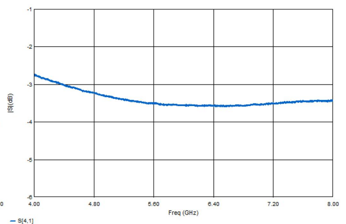
Figure 4. MHC60X03 Transmission
