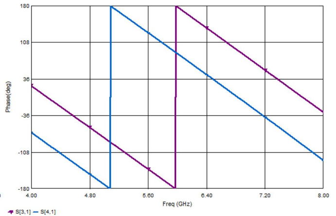
Figure 10. MHC60X03 Phase
