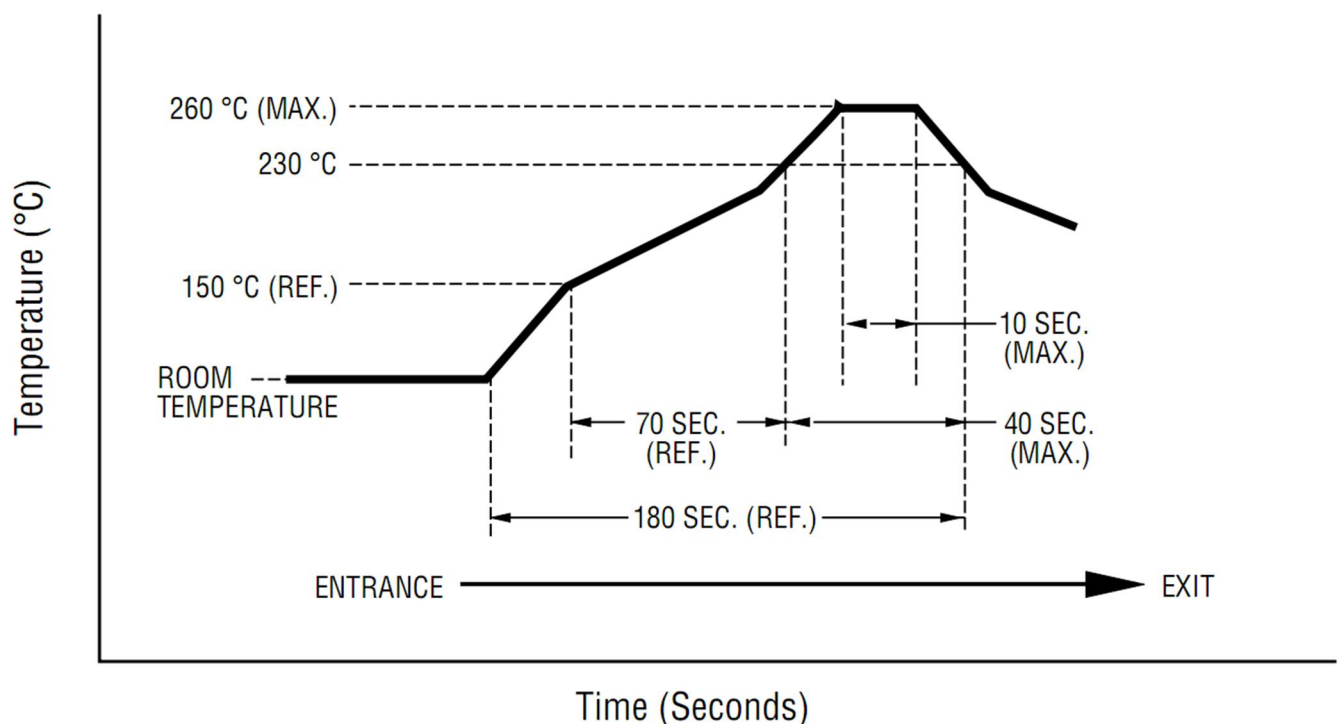
Figure 11. MHC60X03 Thermal Reflow Profile
