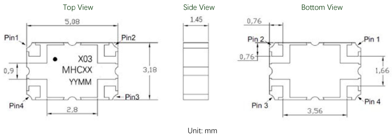
Figure 2. MHC60X03 Outline Drawing
