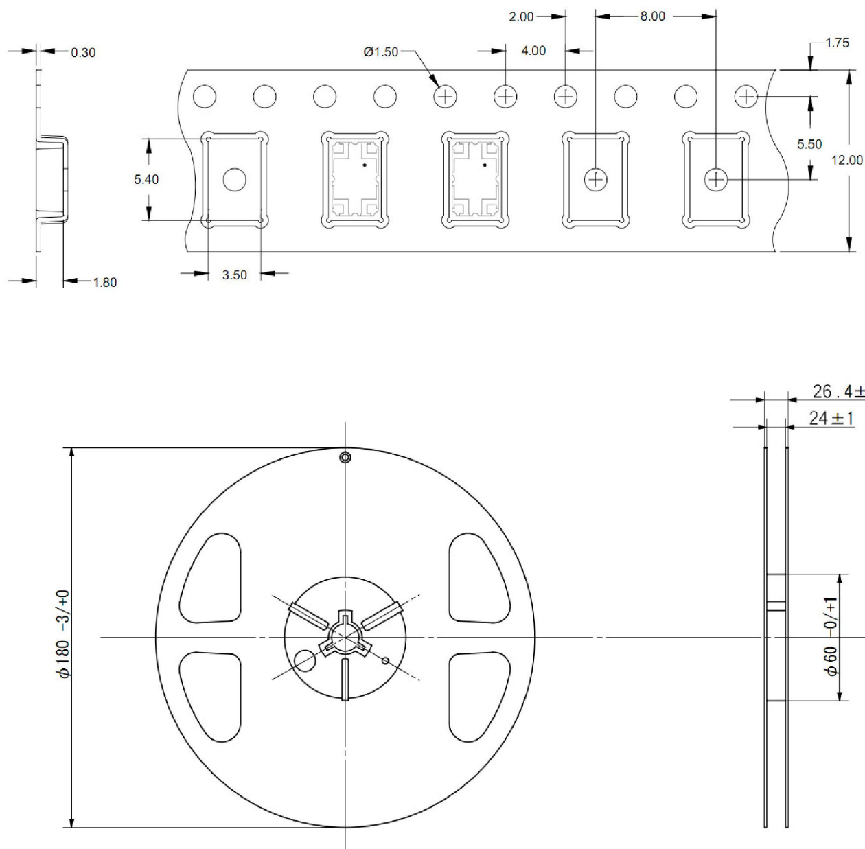
Figure 12. MHC60X03 Packaging Information
