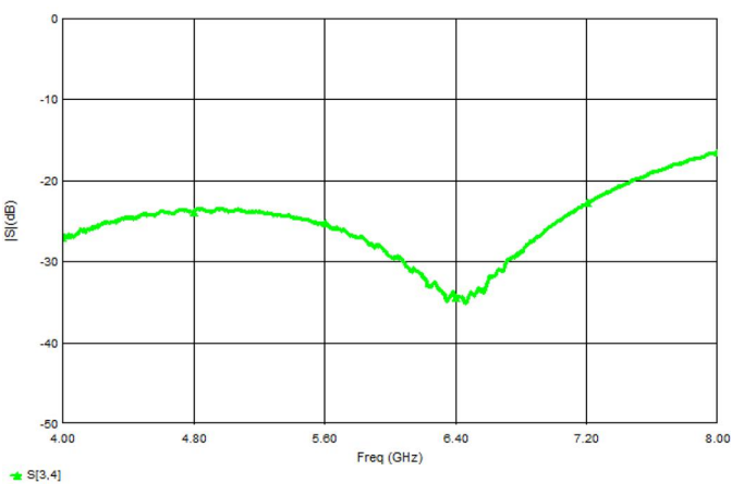
Figure 9. MHC60X03 Isolation
