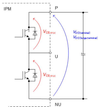
Fig.2-2 Rated Voltage
