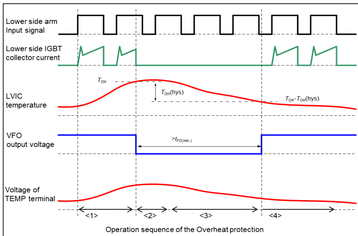
Fig.2-7 Overheat Protection
