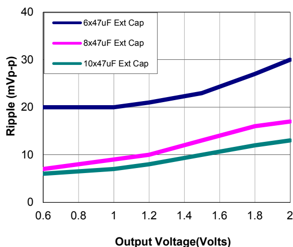
Fig-2: Output ripple voltage for various output voltages with external 6x47uF, 8x47uF or 10x47uF ceramic capacitors at the output (40A load). Input voltage is 12V. Scope Bandwidth limited to 20MHz.
