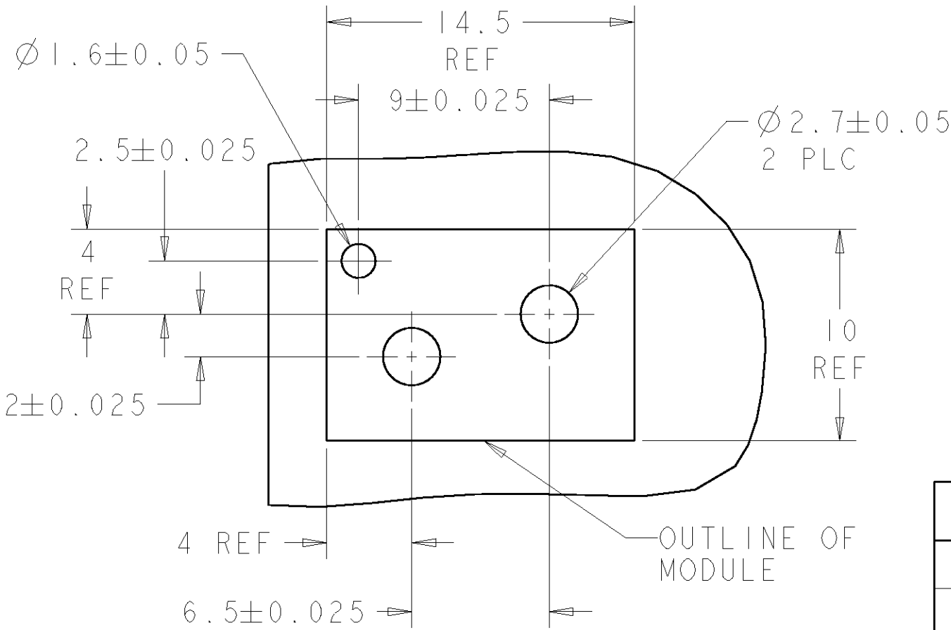
PCB LAYOUT
