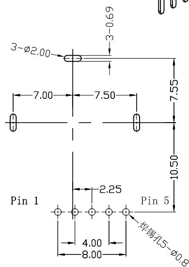
P. C. B MOUNTING HOLE DETAIL
