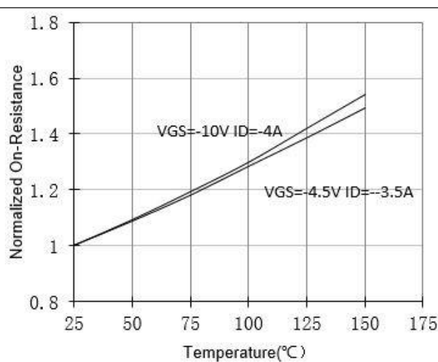
Figure2. On-Resistance vs. Junction Temperature
