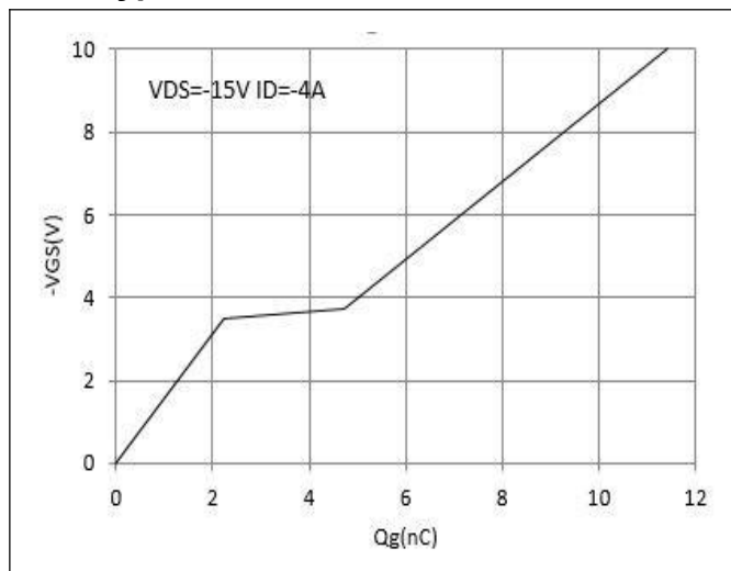
Figure 7. Charge Characteristics
