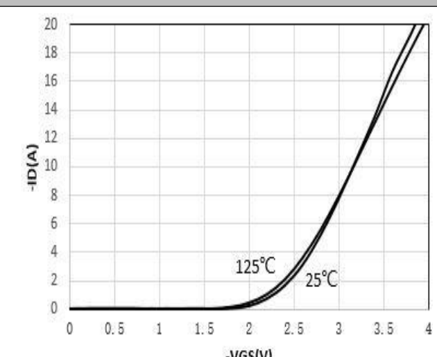
Figure 6. Transfer Characteristics
