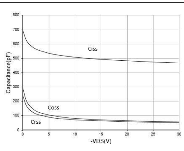
Figure 8. Capacitance Characteristics
