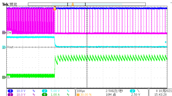
Figure 15. Over Current Protection(100mA to hard short)
