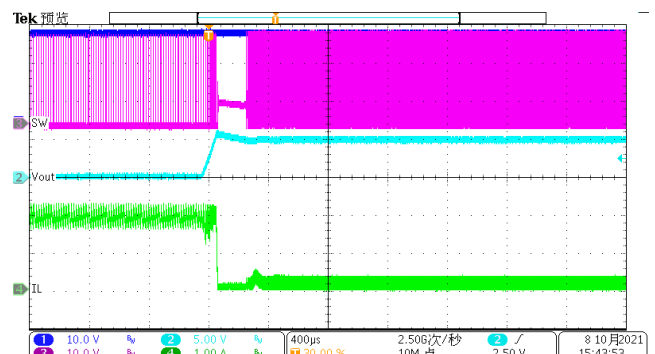
Figure 16. Over Current Release (hard short to 100mA)
