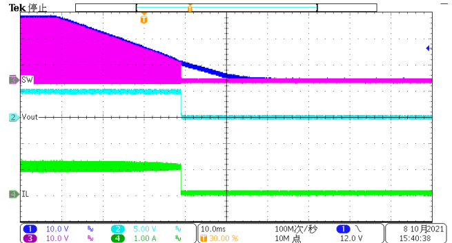
Figure 12. Power down(Iload=1A)
