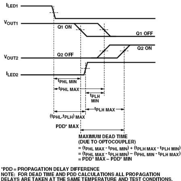
Figure 28 Waveforms for Dead Time
