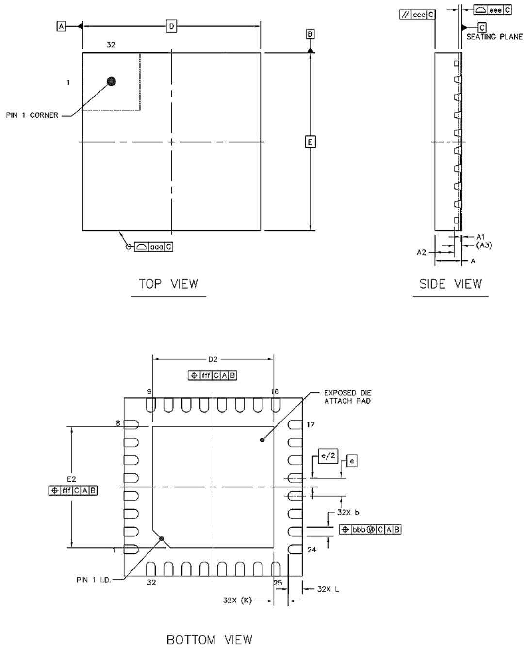
Figure 17. Mechanical Information
