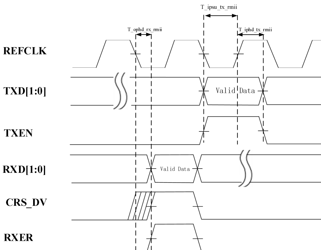
Figure 13. RMII2 Transmission and Reception Cycle Timing
