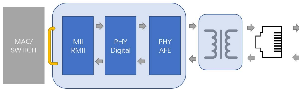
Figure 8. Remote loopback
