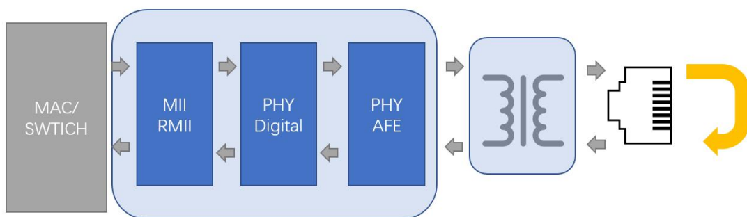
Figure 7. External loopback
