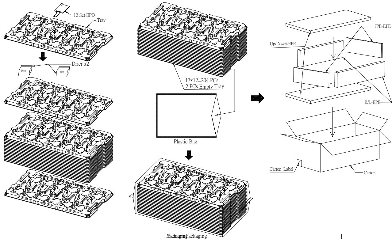
Figure 7-1 Packing Diagram
