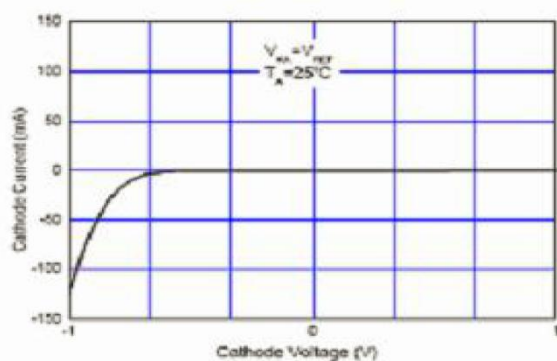
Figure 8. Cathode Current vs. Cathode Voltage
