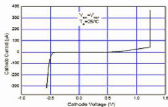
Figure 9. . Current vs. cathode Voltage
