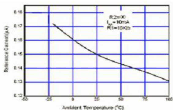
Figure 7. Reference Current vs. Ambient Temperature
