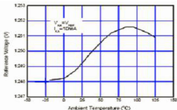
Figure 6. Reference Voltage vs. Ambient Temperature
