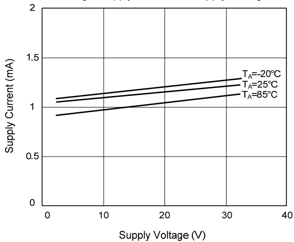
Fig.3 Supply Current vs Supply Voltage
