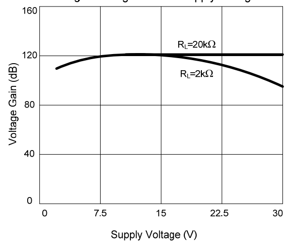
Fig. 4 Voltage Gain vs Supply Voltage
