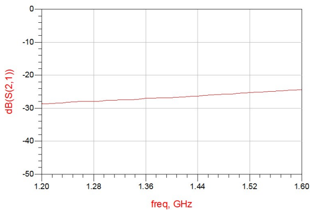
Figure 9. MHC1400L03 Isolation
