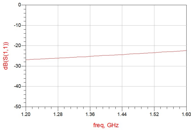
Figure 5. MHC1400L03 Return Loss (S11)
