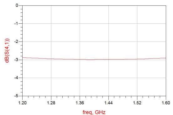
Figure 4. MHC1400L03 Transmission
