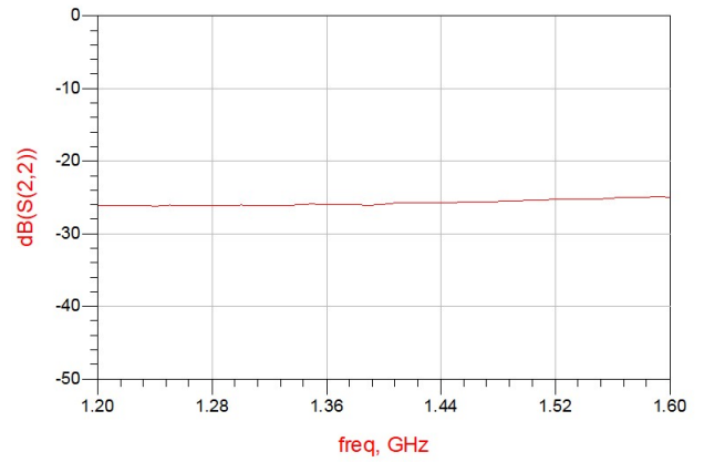
Figure 6. MHC1400L03 Return Loss (S22)
