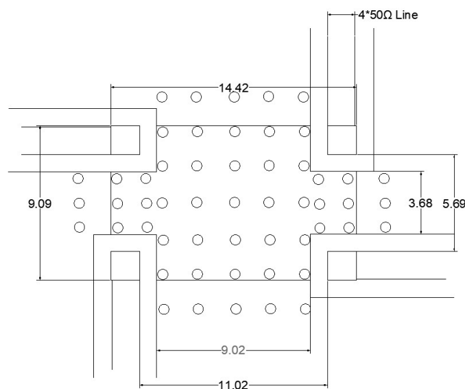
Figure 11. Recommended PCB Layout
