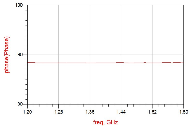
Figure 10. MHC1400L03 Phase
