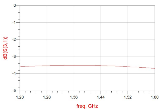
Figure 3. MHC1400L03 Coupling
