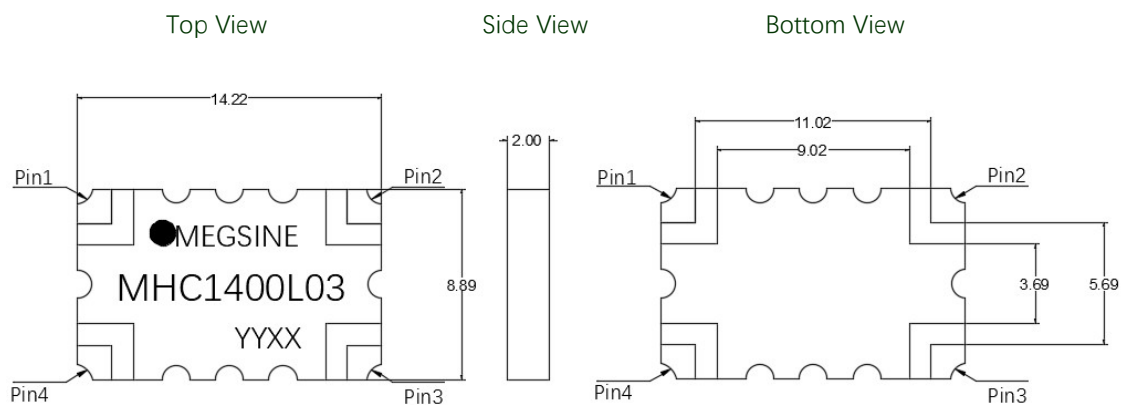
Figure 2. MHC1400L03 Outline Drawing
