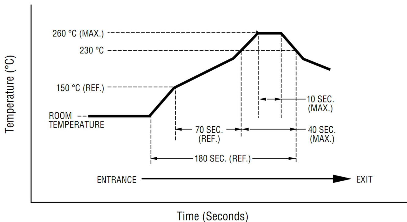
Figure 12. MHC1400L03 Thermal Reflow Profile
