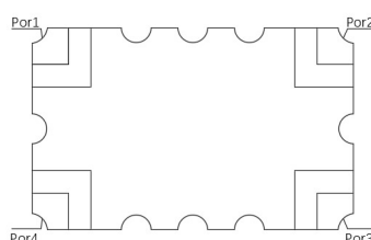
Figure 1. MHC1400L03 (Bottom View)
