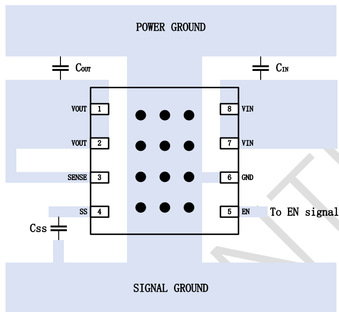
Figure 10.1. Fixed output
