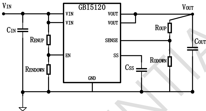
Figure 5.1. Typical Application
