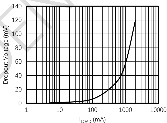
Dropout Voltage vs. Load Current ( I_{LOAD} ), V_{OUT}=5\text{V}
