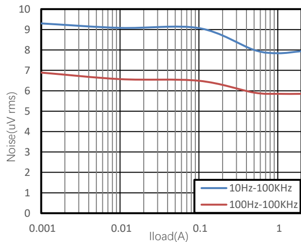
RMS Output Noise vs. Load Current (ILOAD), Vout = 5V
