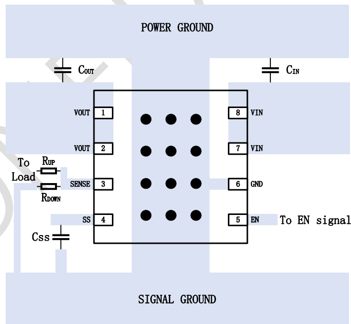
Figure 10.2. Programmable output
