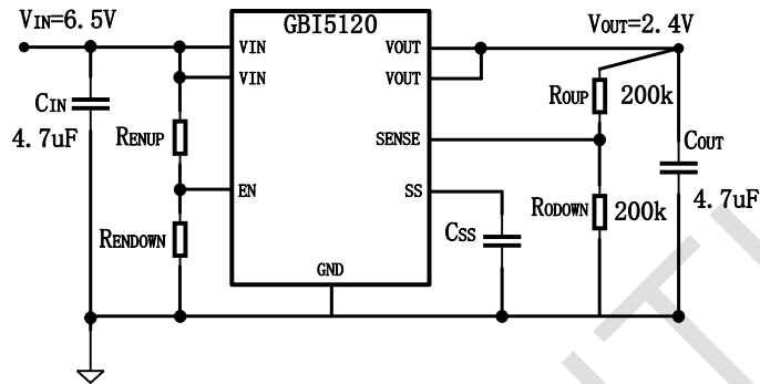
Figure 8.2. Typical Adjustable Output Voltage Application Schematic
