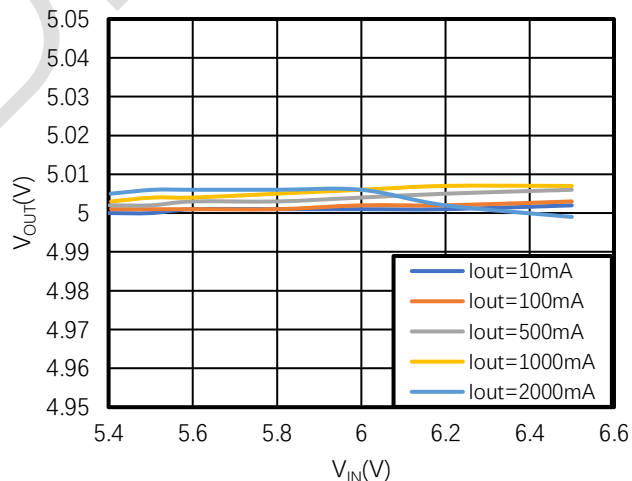
Output Voltage vs. Input Voltage ( V_{IN} ) in Dropout V_{OUT} = 5 V
