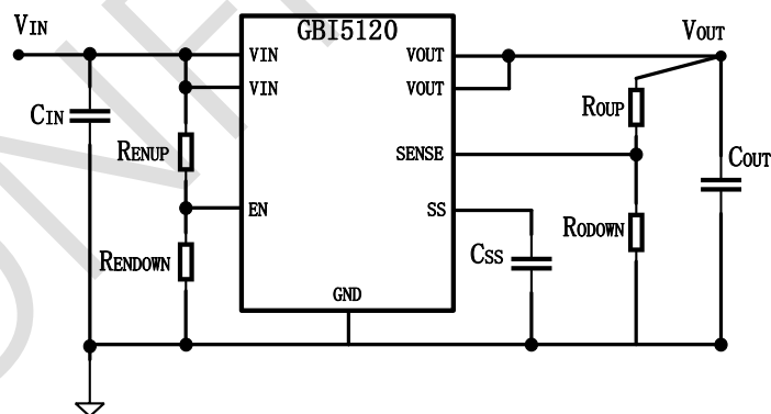
Figure 9.1. Typical Application
