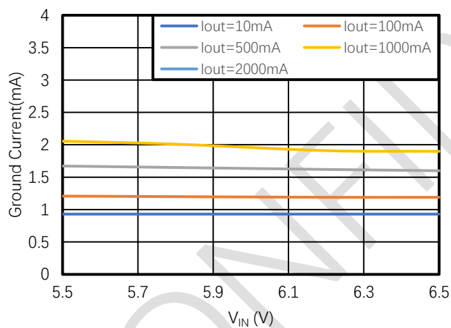
Ground Current vs. Input Voltage ( V_{IN} ), V_{OUT} = 3V
