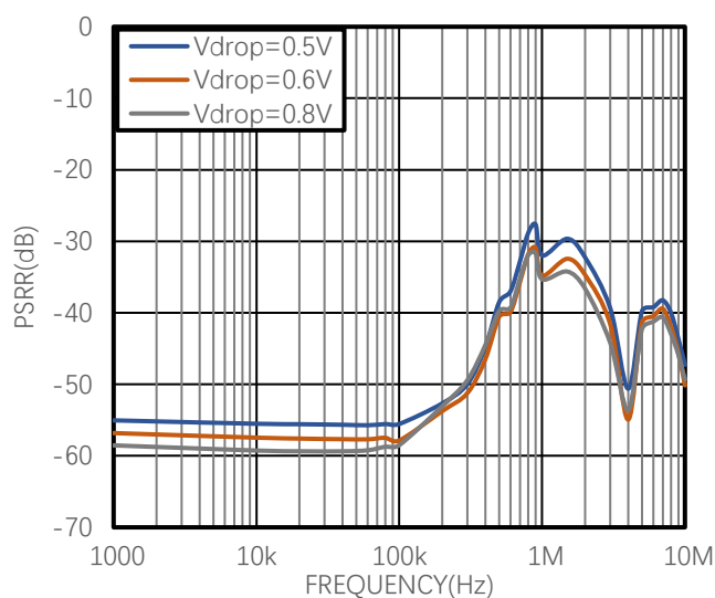
PSRR vs. Frequency, I_{out}=1\text{A} , V_{out}=3\text{V}
