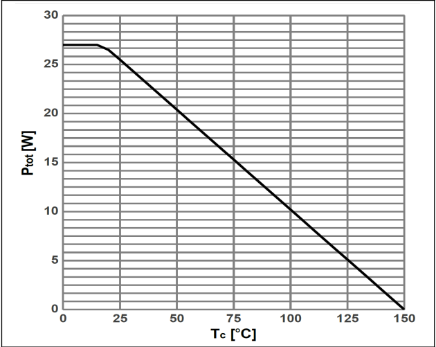
Figure 4: Power dissipation For TO-220、TO-252、TO-263
