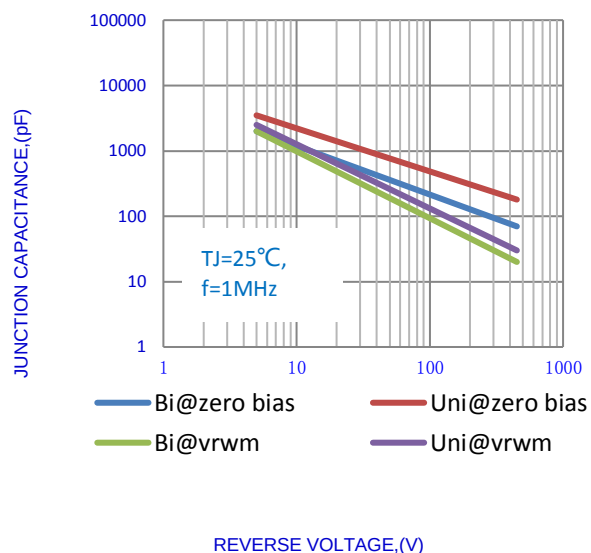
Fig.4-TYPICAL JUNCTION CAPACITANCE
