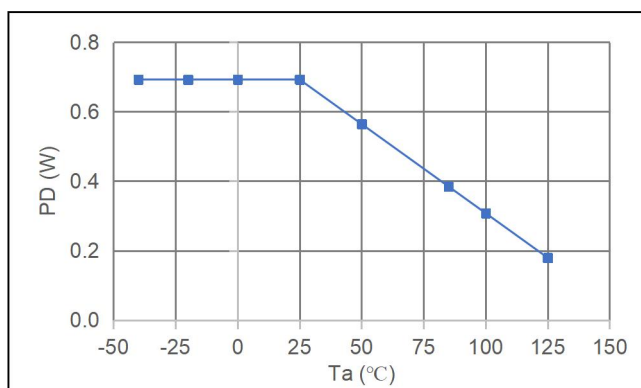
Power Dissipation of SOT335
