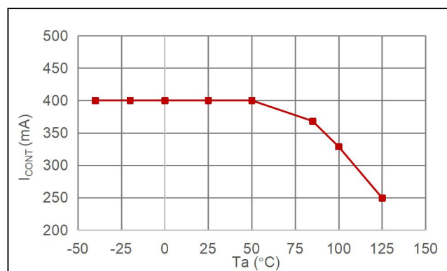
Maximum Output Current SOT335
