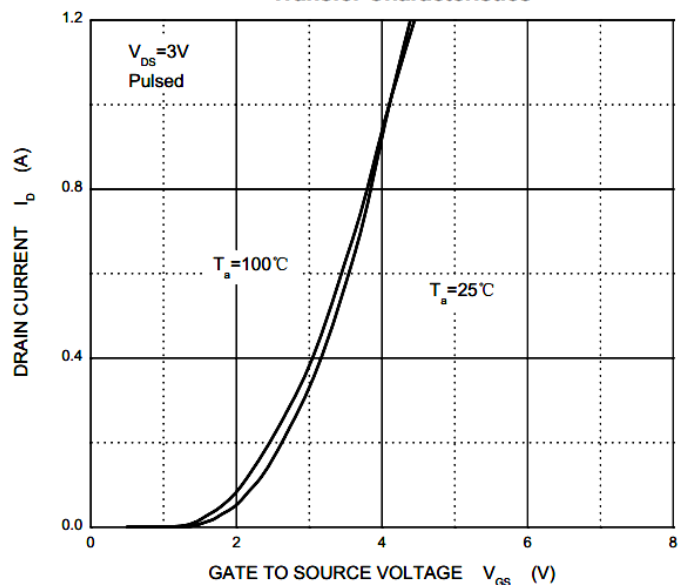
Transfer Characteristics
