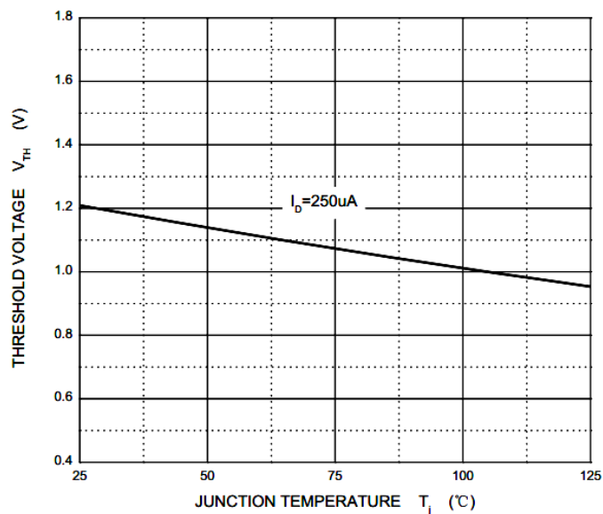
Threshold Voltage
