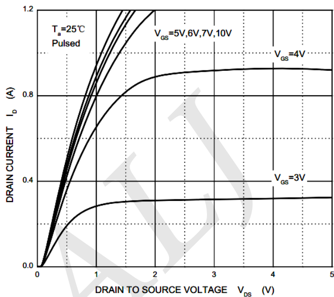
Output Characteristics
