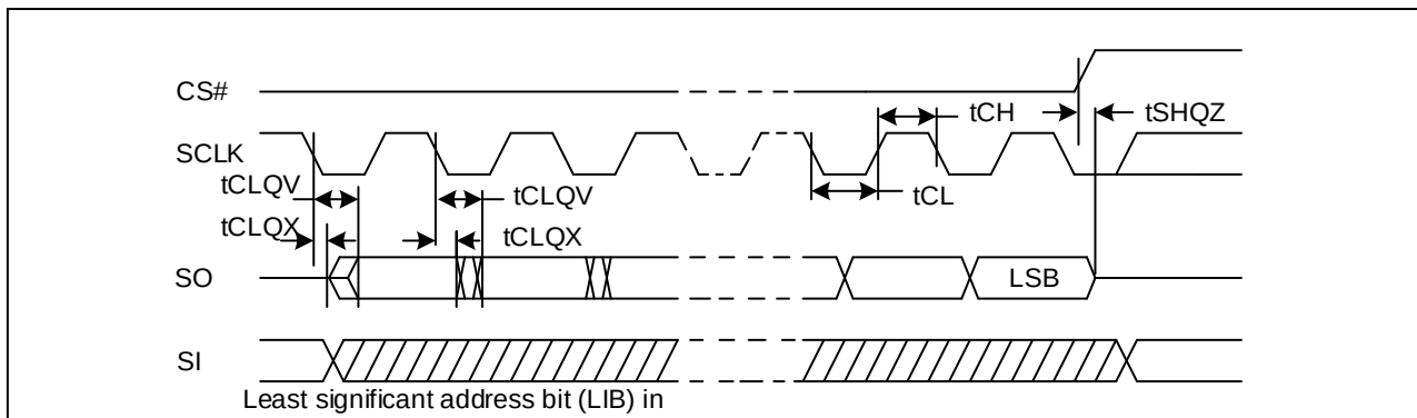
Figure 18-2. Output Timing
