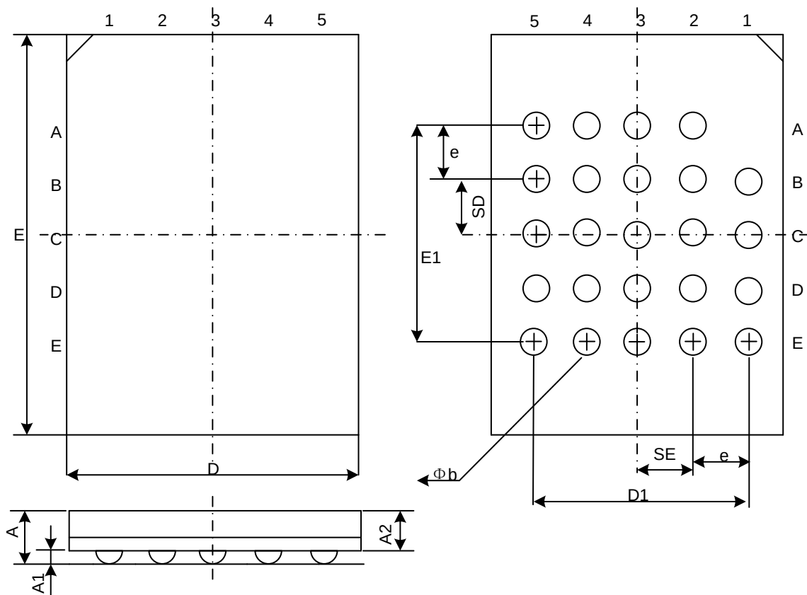
Figure 20-3.TFBGA-24BALL (5*5-1 ball array)
