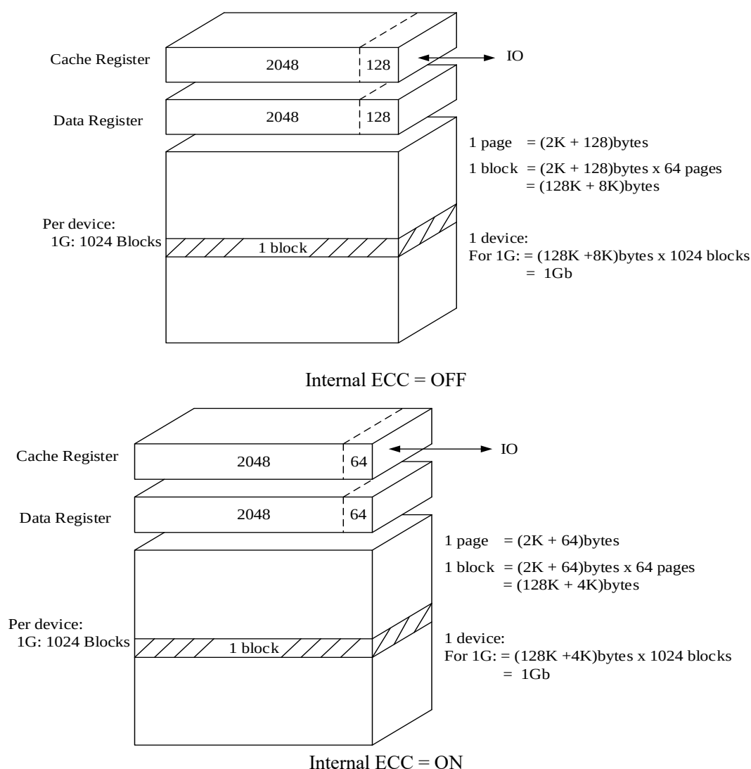
Figure 3. Array Organization
